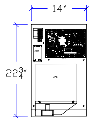
CPU ENCLOSURE (14"W x 22 3 / 4 "H x 4"D)
